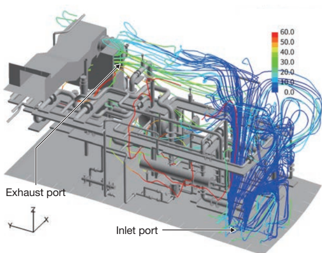
Fig. 3 Ventilation flow analysis for cargo machinery room
