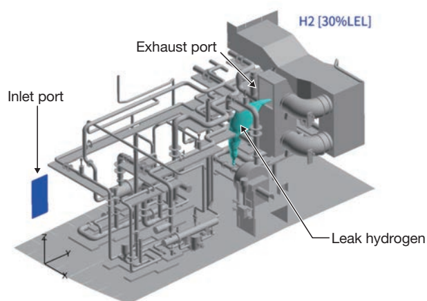
Fig. 4 Hydrogen leakage behavior analysis for cargo machinery room
