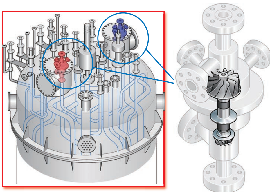
Fig. 3 Hydrogen liquefier (upper part) and expansion turbine
