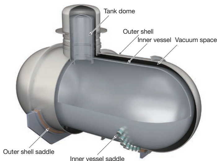
Fig. 2 CCS's double-shell structure
