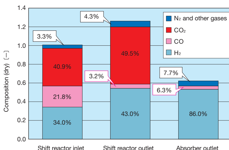
Fig. 6 Results of bench scale test — chemical absorption method
