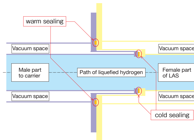
Fig. 3 Bayonet joint
