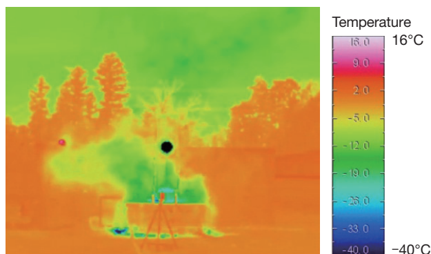
(b) Temperature distribution of liquefied hydrogen
