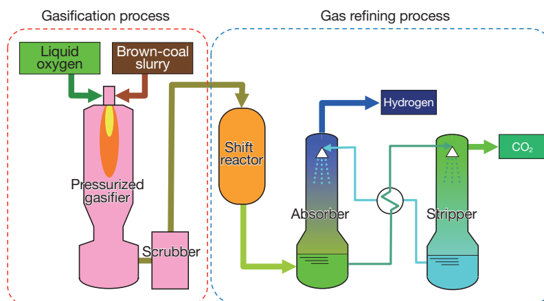
Fig. 3 Process of producing hydrogen by brown-coal gasification
